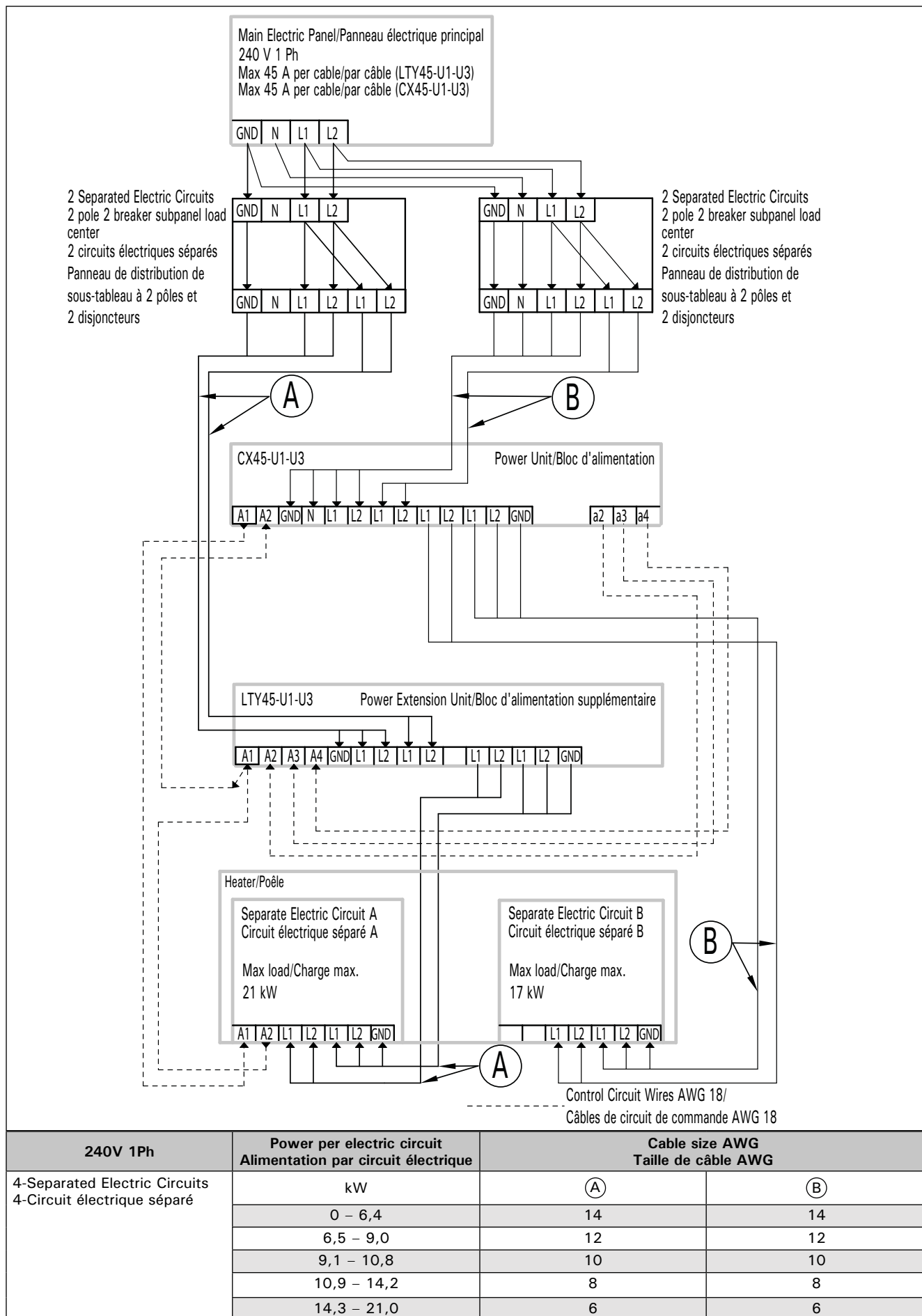
Figure 9. Connection of power extension unit LTY45-U1 with control unit CX45-U1 (240 V / 1Ph, Two separated electric circuits between power extension unit and heater).
