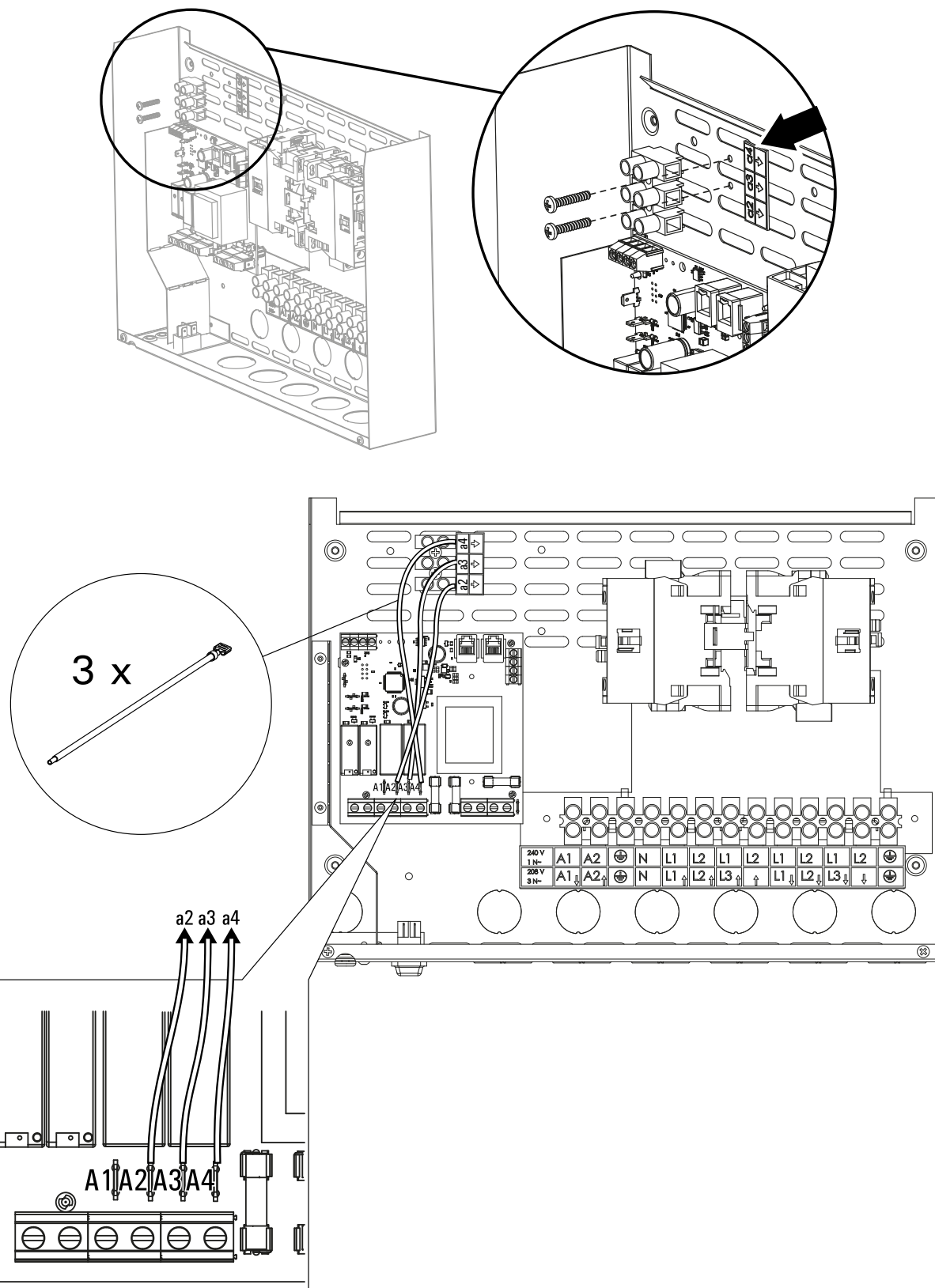
Figure 3. Installation and connection of additional terminal block and adhesive label inside the power unit CX30-U1-U3 / CX45-U1-U3
