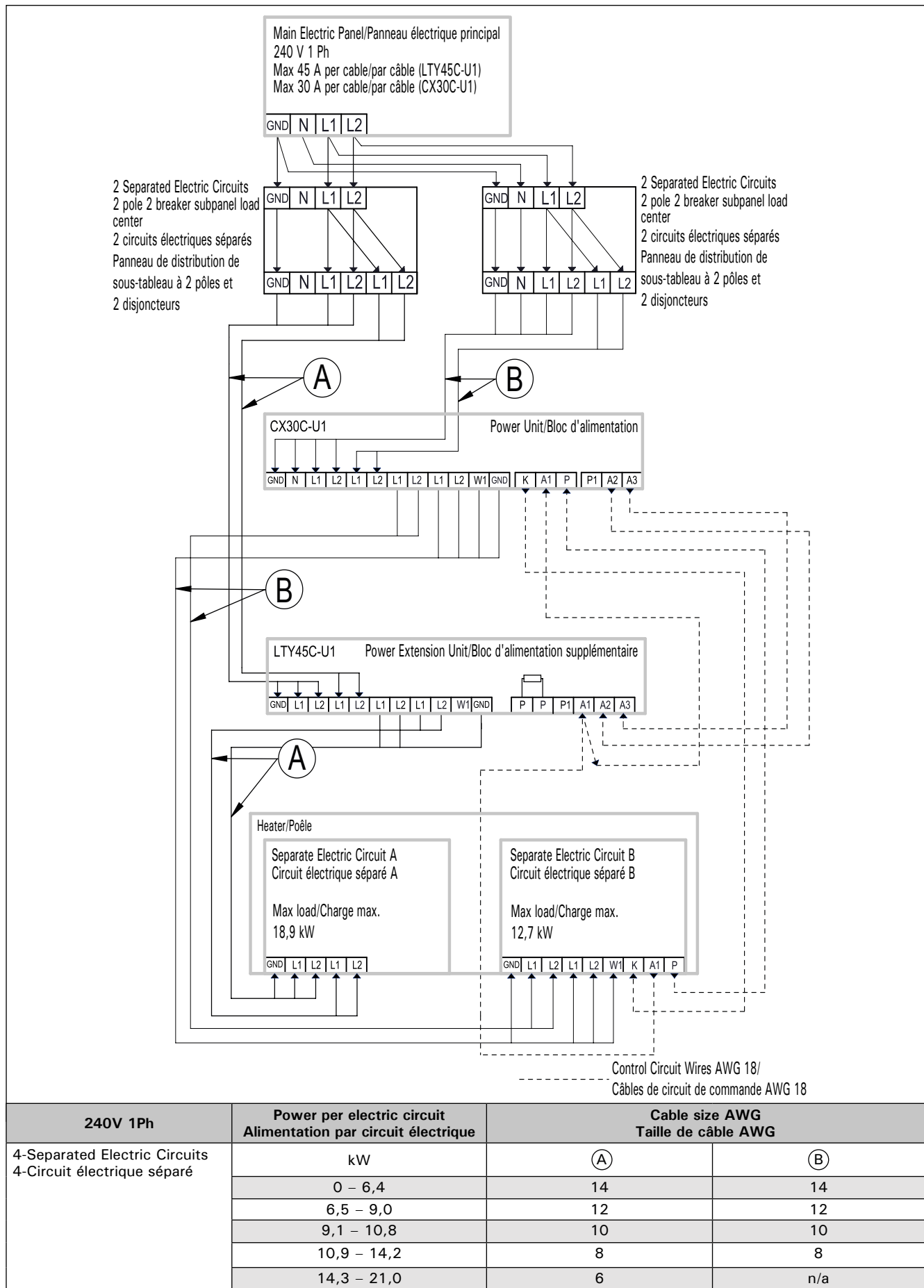
Figure 17. Connection of power extension unit LTY45C-U1 with control unit CX30C-U1 (240 V / 1Ph (Two separated electric circuits between power extension unit and heater). Heater with one built-in steamer units and without one pair of A1/A2 terminals
