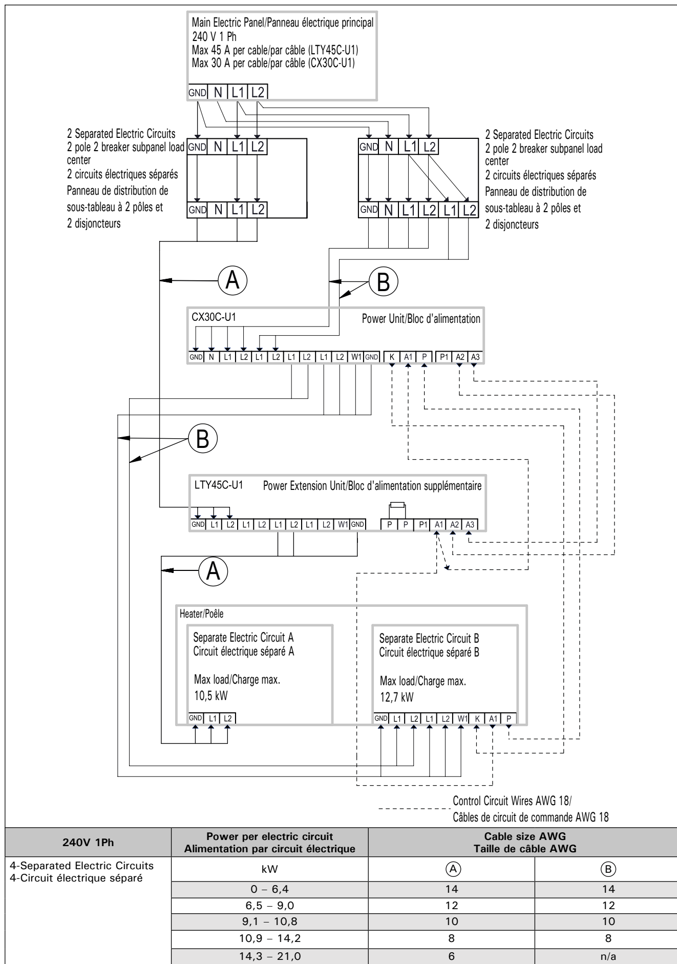
Figure 19. Connection of power extension unit LTY45C-U1 with control unit CX30C-U1 (240 V / 1Ph) Heater with one built-in steamer units and without one pair of A1/A2 terminals
