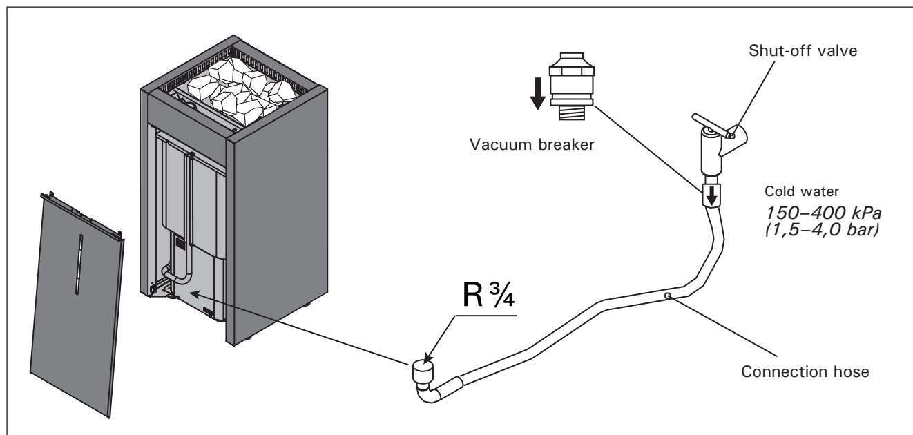
Figure 7. Automatic filling
